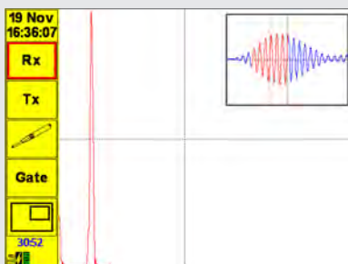
Frequency Spectrum Plot with Inset RF Trace showing Gate Area
