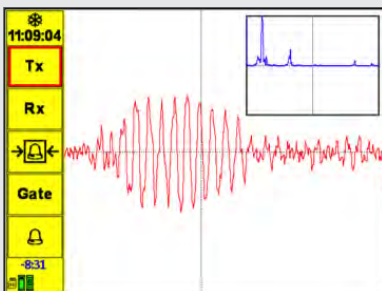
RF (A-Scan Waveform) with Frequency Spectrum Inset
